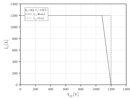
反偏安全工作区 IGBT, 逆变器 (RBSOA) Reverse bias safe operating area IGBT, Inverter(RBSOA)
